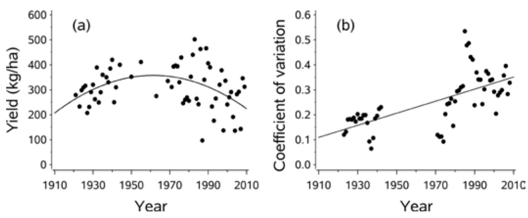
Figure 3. Trends in red clover seed yields in the last 90 years. (a) Yearly statistic of yield per hectare. (b) Variability in yield presented as the coefficient of variation calculated from 5 year moving average (with minimum four values), (reprinted from Bommarco et al., Proc. Roy. Soc. B.).
